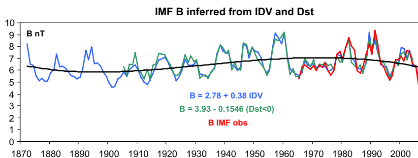
Fig. 6. The magnitude B of the interplanetary magnetic field near the earth observed by spacecraft (red curve) and inferred from the IDV -index (blue curve and regression formula). The green curve shows B calculated from an extension (Love, 2006) back to 1905 of the Dst -index computed using only the negative values. (For interpretation of the references to color in this figure legend, the reader is referred to the web version of this article.)
