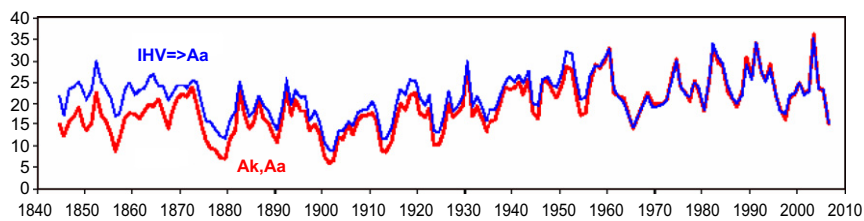
Fig. 14. Comparison between the aa -index back to 1868 and the ak -index (red) extension thereof (derived by Nevanlinna and Kataja (1993)) and our IHV -index (blue) scaled to aa . The ak -values are generally \sim 6 nT lower. (For interpretation of the references to color in this figure legend, the reader is referred to the web version of this article.)
