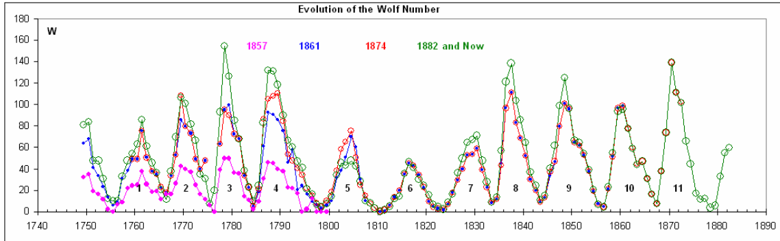
Figure 2. Evolution of the Wolf Number from his first 1857 list to the final version, with color coded curves for each list.
