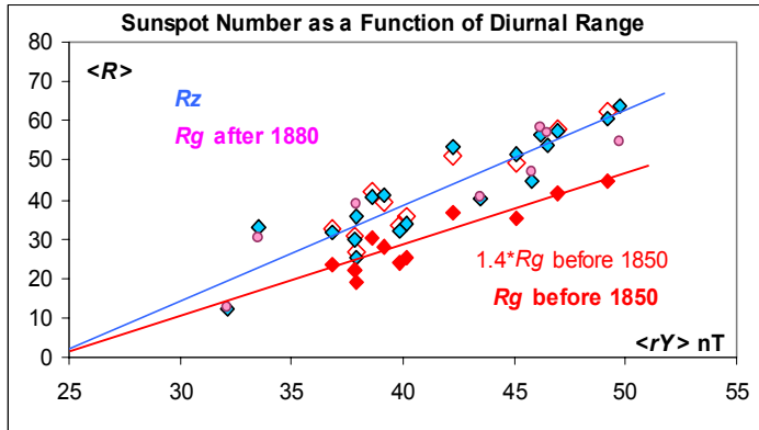
Figure 9. Same as Figure 8, but with the average GSNs for intervals before 1850s added [red filled diamonds]. Scaling these values up by a factor of 1.4 [open red diamonds] brings them into fair agreement with the common regression line for the Wolf SSNs and for the GSNs after 1880.
