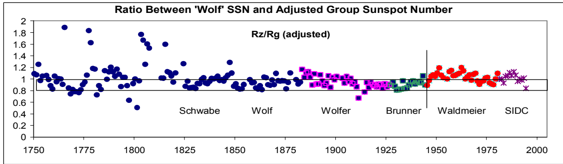
Figure 11. The ratio of yearly values of the Wolf [Zürich] Sunspot Number, R_z , and the Group Sunspot Number, R_g . Different observers are indicated by appropriate color coding.
