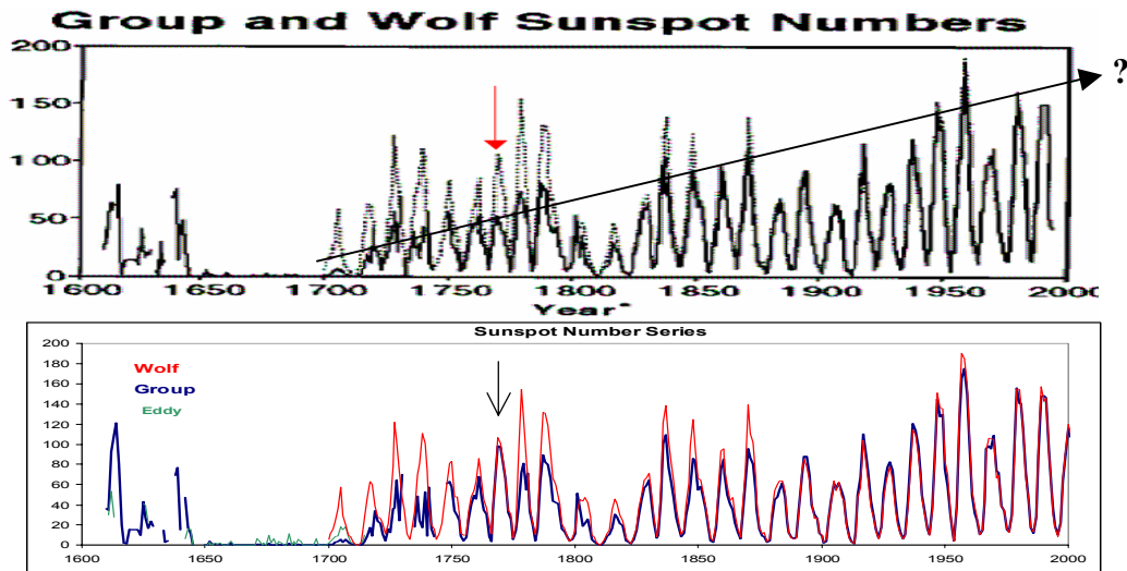
Figure 6. Two versions of the GSN [top: GSN full line, Wolf SSN dotted line]. The latest GSN compared to the Wolf [and International] SSNs in the bottom panel. The GSN is largely based on the RGO [Greenwich] dataset from 1875 onwards.
