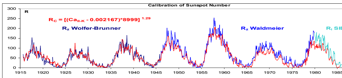
Figure 14. Comparison of Zurich SSN [blue colors] and a synthetic SSN [red] calculated from a Ca II K-line index using a pre-Waldmeier relationship.
