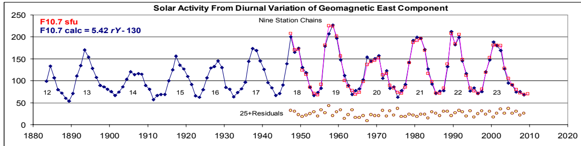
Figure 15. The yearly average range, rY, derived from nine long-running chains of geomagnetic observatories [blue] compared with the average F10.7 cm solar flux [red].
