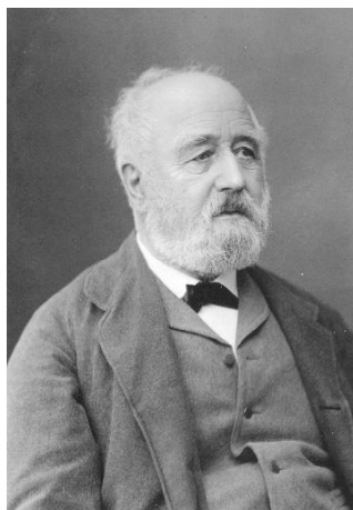
Figure 1. Rudolf Wolf and excerpts from his 1861 list of published Relative Numbers compared with his latest list (now the official list from SIDC in Brussels).
