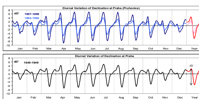
Figure 4. Diurnal variation of Declination at Prague per month. Top: modern data for low sunspot number [light blue] and for high sunspot number [dark blue]. Bottom: for the 1840s. The amplitude changes with the solar zenith angle. Wolf used the yearly average [red] to calibrate the yearly R_W .
