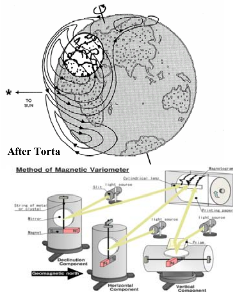
Figure 3. Ionospheric current system fixed with respect to the Sun. Stations rotate into and out of the magnetic field of this system, recording it.
