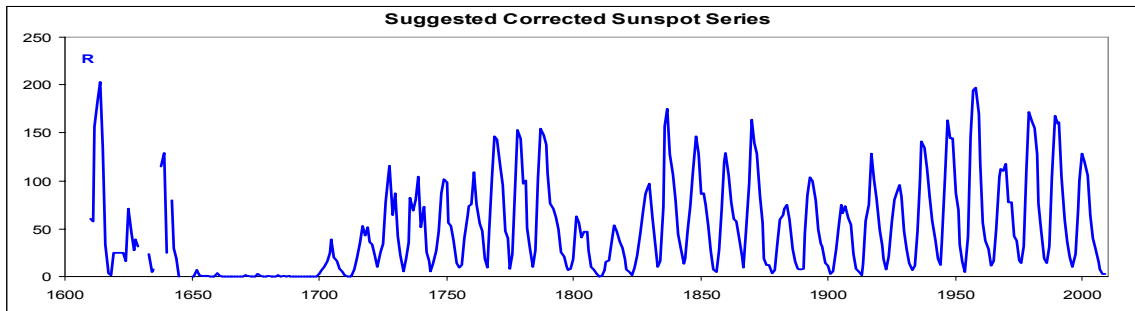
Figure 16. Suggested equivalent sunspot numbers calibrated by the geomagnetic record.
