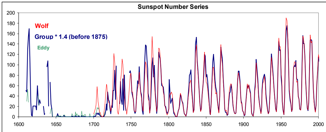
Figure 10. The GSN adjusted upwards by a factor of 1.4 before 1875 (blue) compared with the Wolf SSN (red).
