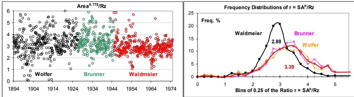
Figure 13. Monthly values of the ratio between the sunspot areas [to power p = 0.775 ] for different observers as indicated.
