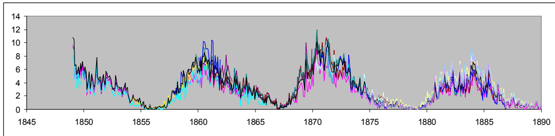
Figure 5. Group counts by several observers: Schwabe, Wolf, Carrington, Shea, Peters, Spörer, Weber, Schmidt, Secchi, Bernaerts, Wolfer, Aguilar, Ricco, and RGO, shown with different color coding.
