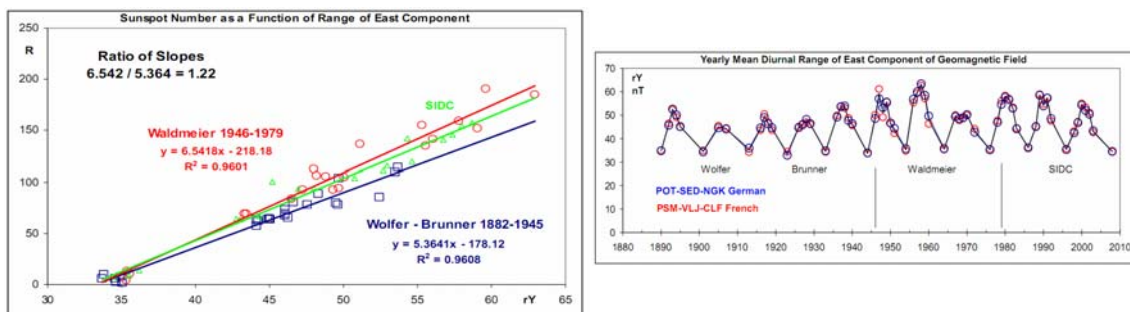
Figure 12. Select years near solar minimum and near solar maximum, then plot the yearly Zürich SSN as a function of the range of the East component for two station chains
