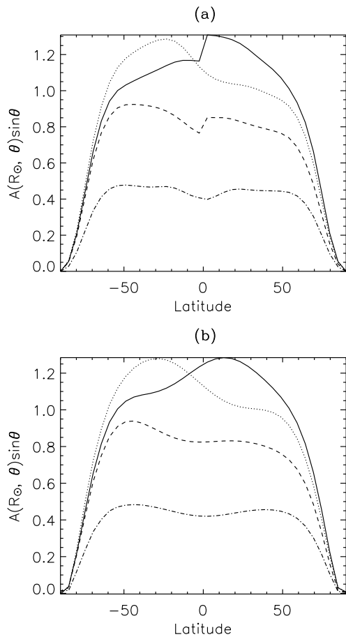
Figure 12. Poloidal field A(R_{\odot}, \theta) \sin \theta inferred from the WSO data (a) before smoothing and (b) after smoothing, for the minima at the ends of cycles 20 (solid line), 21 (dotted line), 22 (dashed line) and 23 (dot-dashed line). It may be noted that A(R_{\odot}, \theta) \sin \theta during the minima at the ends of cycles 21 and cycle 23 is negative. We have plotted the absolute values.
