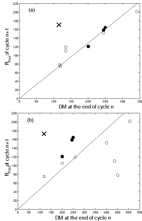
Figure 2. Strengths of solar cycles plotted against the DM values of polar fields at the preceding minima. The solid circles are based on actual polar field measurements whereas the open circles are based on polar fields inferred (a) from values of A(t) at the minima as given by Makarov et al. (2001), and (b) from the numbers of polar faculae at the minima as given by Sheeley (1991). The points marked by ‘x’ and ‘□’ indicate the data points for cycle 24 according to the models of Dikpati & Gilman (2006) and CCJ.
