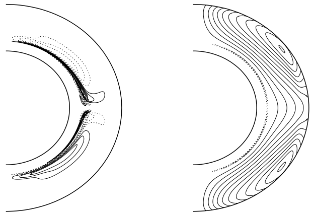
Figure 14. (a) The contours of toroidal field and (b) the poloidal field lines, at the solar minimum in an undisturbed run of our Standard1 model. The solid lines indicate positive values of B and A , whereas dotted lines indicate negative values.
