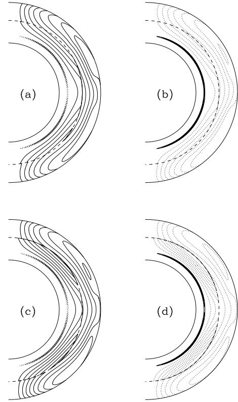
Figure 15. The poloidal field lines given by constant contours of A \sin \theta just after correcting by the observational data during the minima at the ends of cycles (a) 20, (b) 21, (c) 22 and (d) 23. The dashed lines correspond to r = 0.8R_{\odot} .
