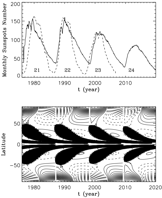
Figure 16. The upper panel shows the theoretical monthly smoothed sunspot number (solid line) superposed on the monthly smoothed sunspot numbers from observation (dashed line). For cycles 22 and 23, the two lines match quite well. But for cycle 21, the result from the model is slightly weaker than the observational result. Incomplete observational data at the end of cycle 20 might be the reason. The cycle 24 is clearly very weak. The lower panel shows the theoretical butterfly diagram of sunspots superimposed on the contours of radial field for the cycles 21–24. The solid and dashed curves in the lower panel indicate positive and negative values of B_r at the surface. (Note that the solid and dashed curves got accidentally interchanged in Fig. 3 of CCJ.)
