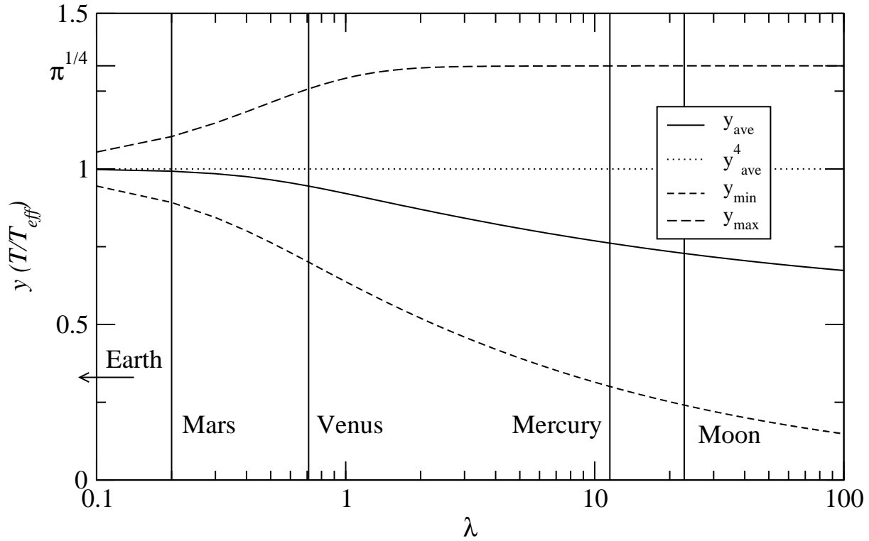
FIG. 2: The average, minimum, and maximum values of the relative temperature y from numerically integrating the equations for different values of \lambda . The numerically computed average value of y^4 is also shown; this should always be exactly 1. Lines are shown indicating the approximate values of \lambda corresponding to the equators of the terrestrial planets, which gives a picture of their most extreme temperature profiles if they had infrared-transparent atmospheres.
