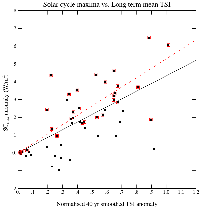
Fig. 6. Solar cycle maxima versus the 40-year smoothed irradiance data from WLS. Linear regression through the origin using all local maxima (solid line) gives SC_{\max}=0.433 (\bar{S}(t_{\max})-\bar{S}(t_{MM}))/\Delta S , ( r^2=0.47 ). Note that a tighter screening of which points count as solar cycle maxima and only using local maxima that exceed the long-term mean (overlain red symbols) gives a slightly steeper regression of 0.53, ( r^2=0.56 ) (dashed line).
