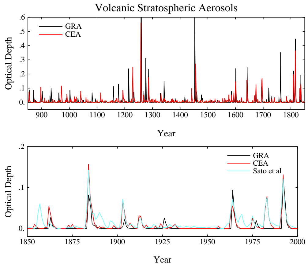
Fig. 4. The two volcanic reconstructions of AOD (at 550 \mu\text{m} ) (GRA and CEA) (top), with a comparison to the modern estimates of Sato et al. (1993) (bottom) (note the different vertical scales in the two panels).
