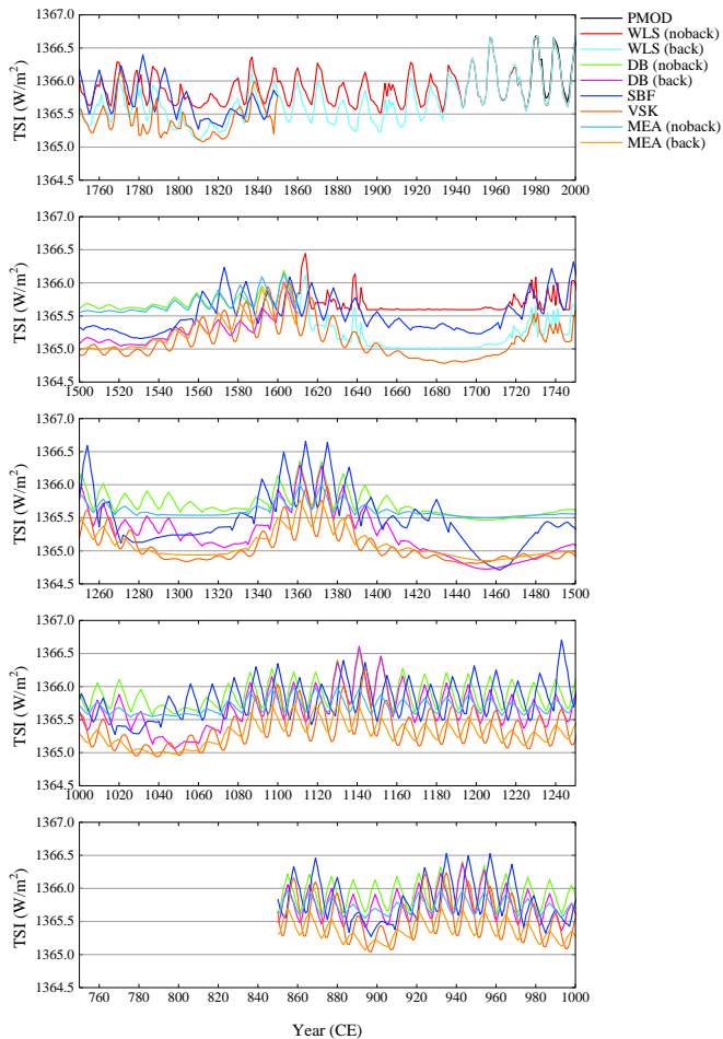
Fig. 8. Multiple TSI reconstructions from 850 CE onwards.
