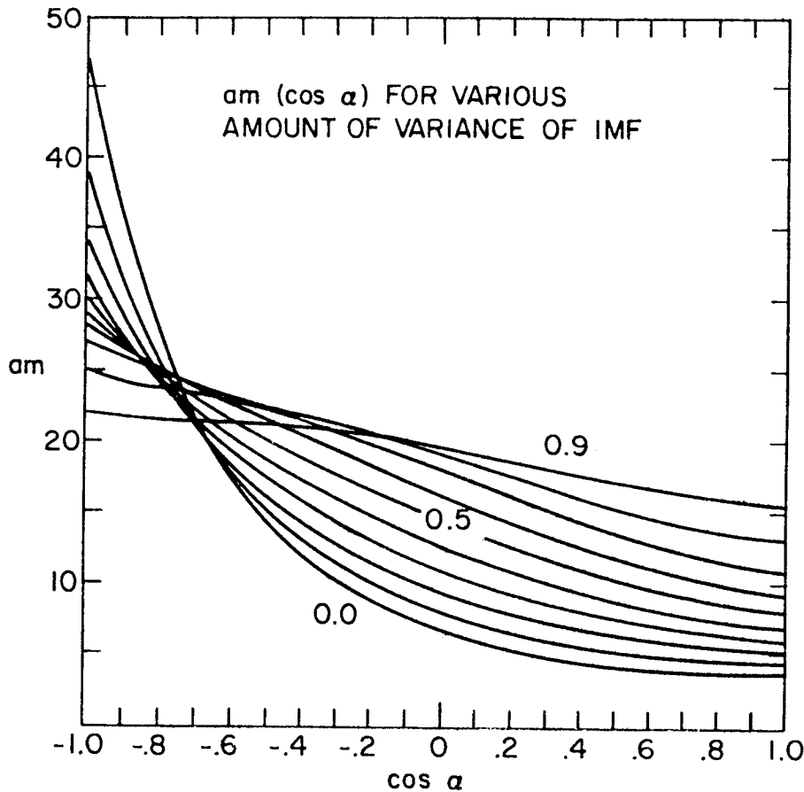
Figure 13. The dependence of geomagnetic activity (am-index reduced for BV and nV^2 influence, see text) on \cos\alpha , where \alpha is the angle between the geomagnetic field lines at the nose of the magnetosphere and the average interplanetary magnetic field during the three-hour interval corresponding to am. Draping (Figure 3) of the interplanetary field is assumed and the reader is referred to Figure 18 for a precise definition of \alpha . Several curves are shown for various values of the relative variability f ; from f = 0.0 to f = 0.9 as labeled on the figure. Note the very flat curves for high variability and the steeply falling curves for low variability of the interplanetary field.
