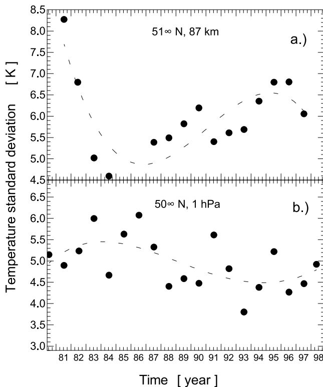
Figure 9. Long-term changes of temperature variability. Annual means of standard deviations are given at (a) 87 km, (51°N, 7°E) and (b) 1 hPa (50°N, 5°E) [from Bittner et al., 2002]. Reprinted with permission from Elsevier.
