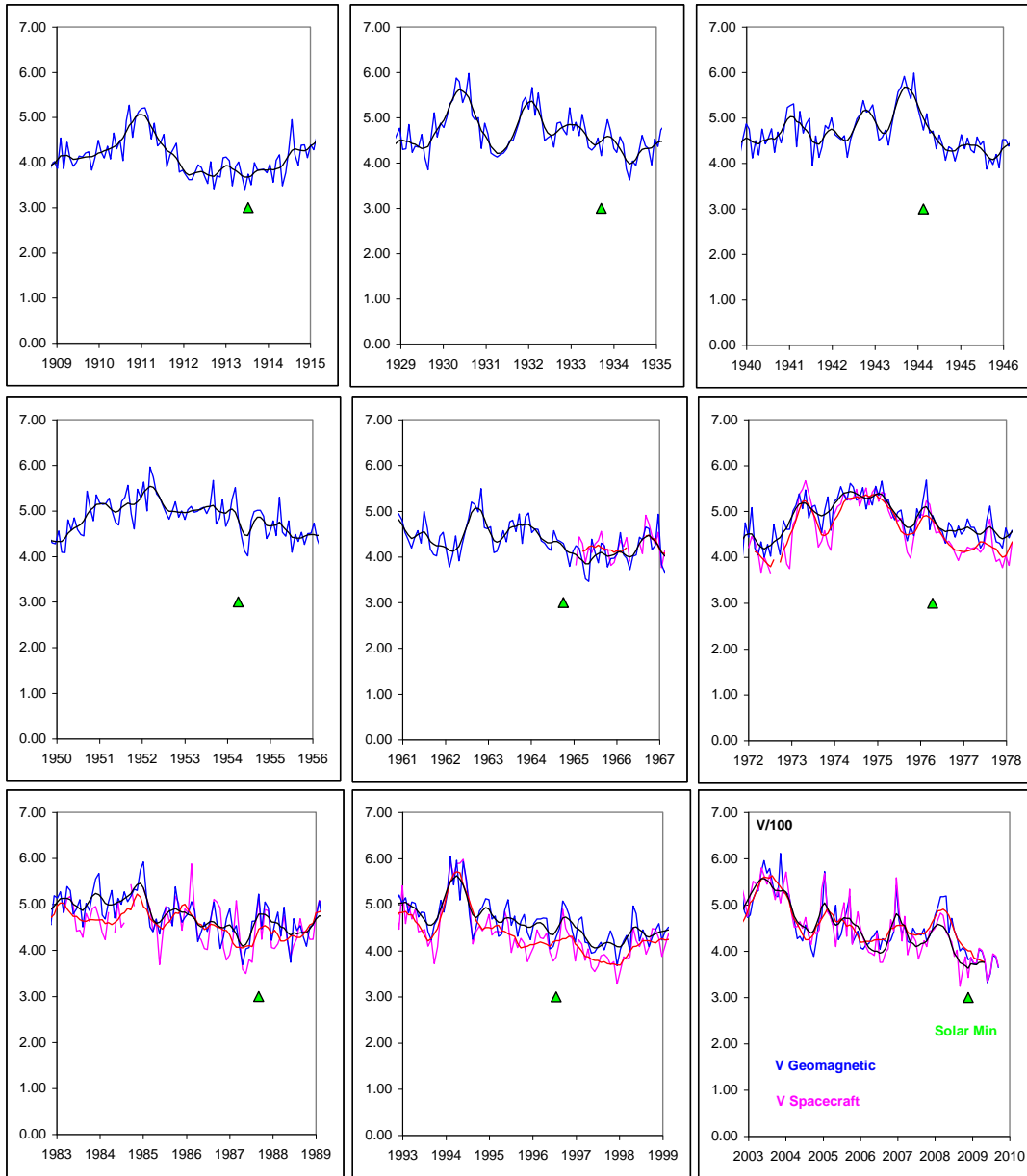
Solar wind speed [in units of 100 km/s] for all solar minima the past 100 years. Blue: inferred from the geomagnetic record, and pink from in situ spacecraft measurements.
