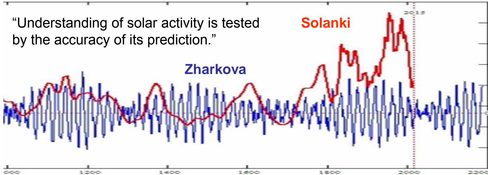
A Millennium of Decadal Sunspot Numbers On St.50 V2 Scale
